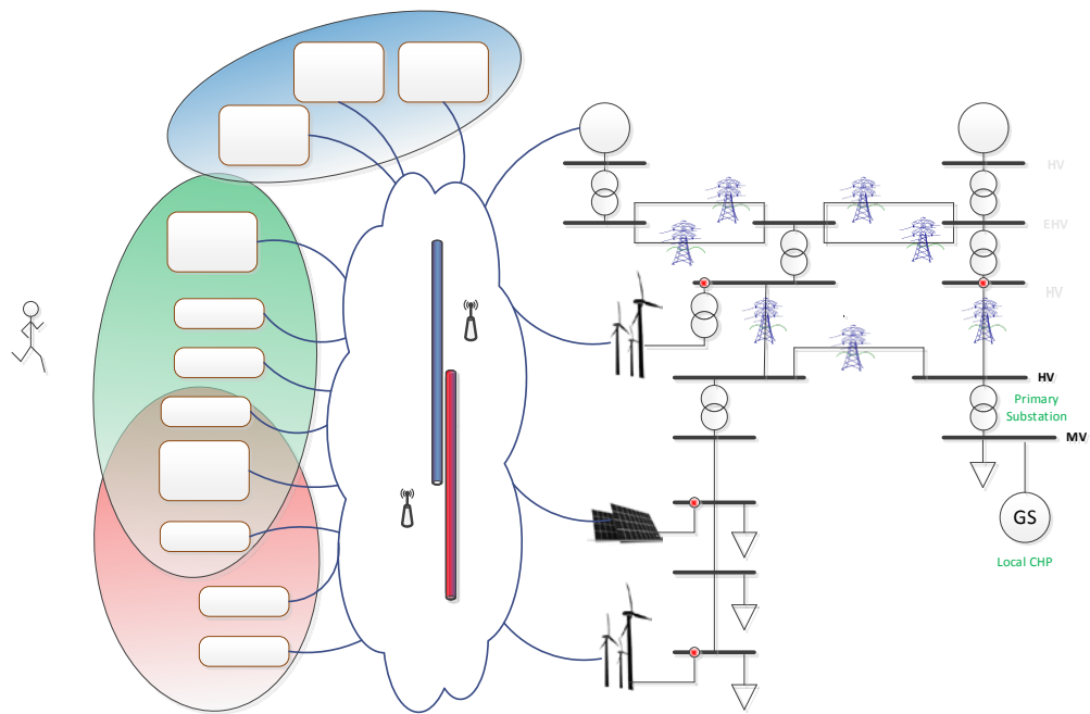
Figure 6: General system architecture including power system & assets, control levels, ICT layer and actors
