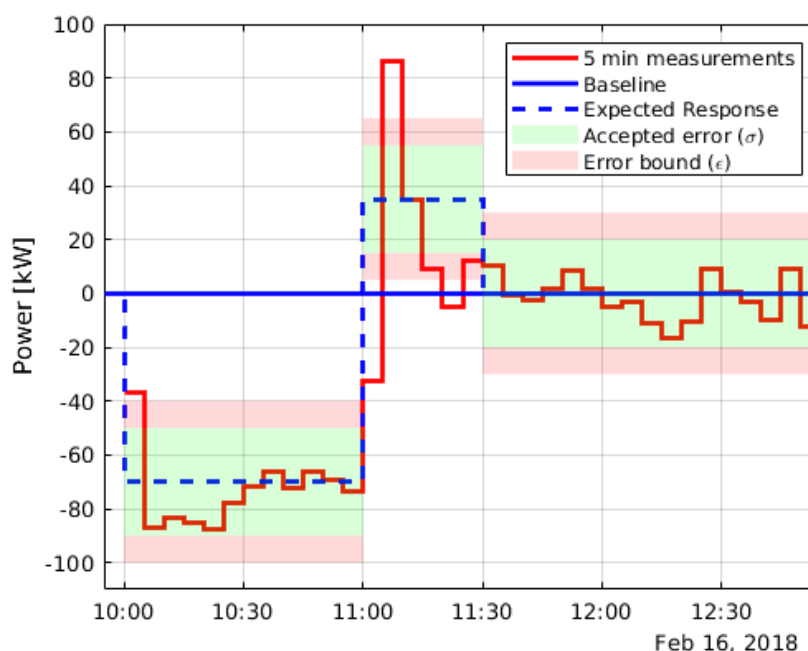
Figure 32. Verification of a specific service delivered on the 16th of February 2018 during heating season 2. This specific service was delivered without rebound control, as rebound control was first implemented in heating season 3.
