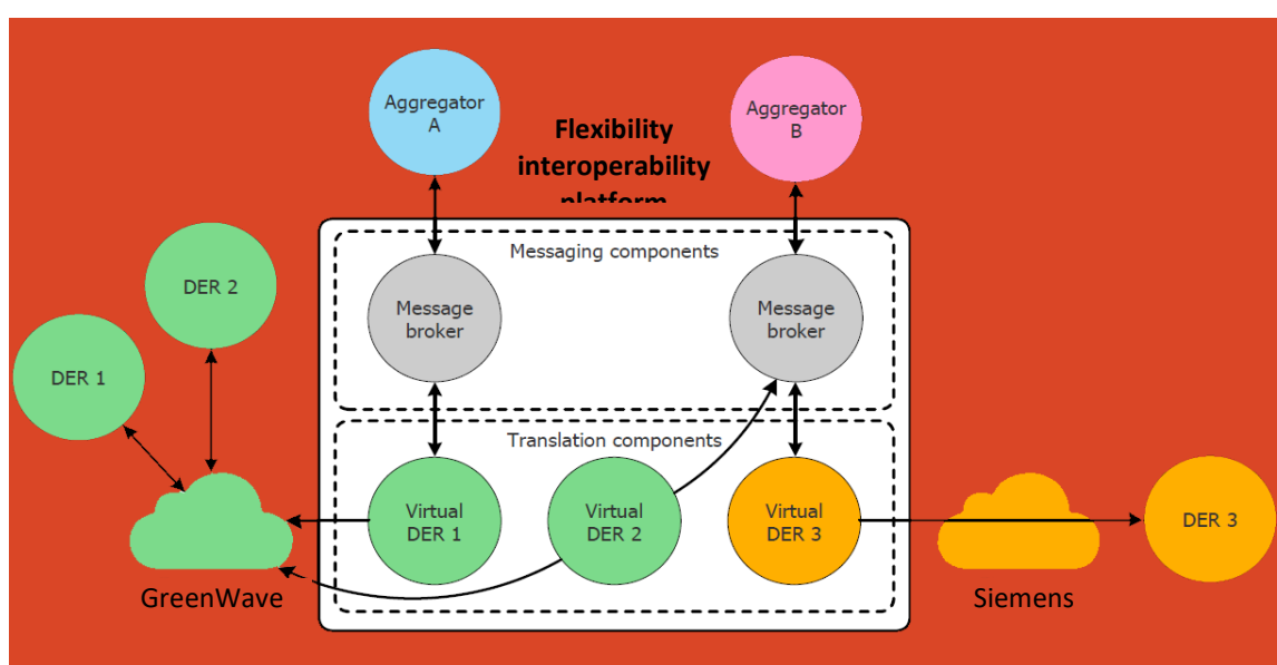
Figure 12. Components of the flexibility interoperability platform.
