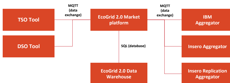
Figure 5. Illustration of market platform.
