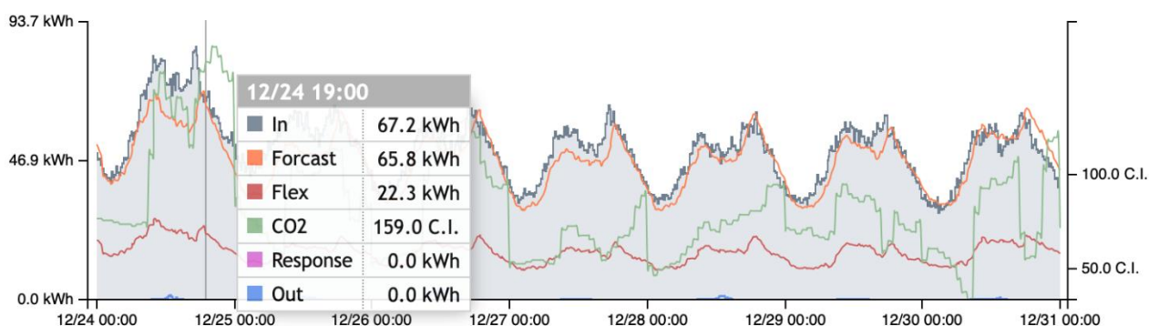
Figure 16. Expected load reduction from 132 electric heating households.
