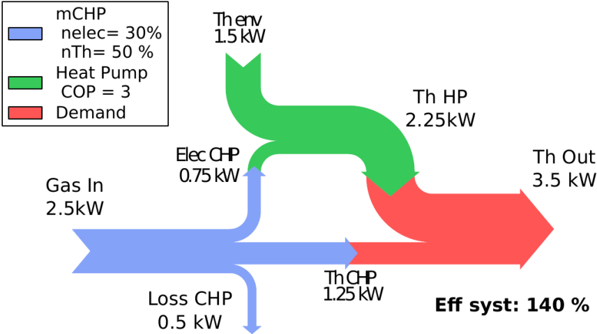
Figure 1: Energy flows in a CHP-HP system
