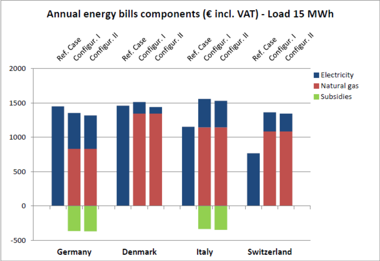
Figure 3: Load 15 MWh –Energy bills components
