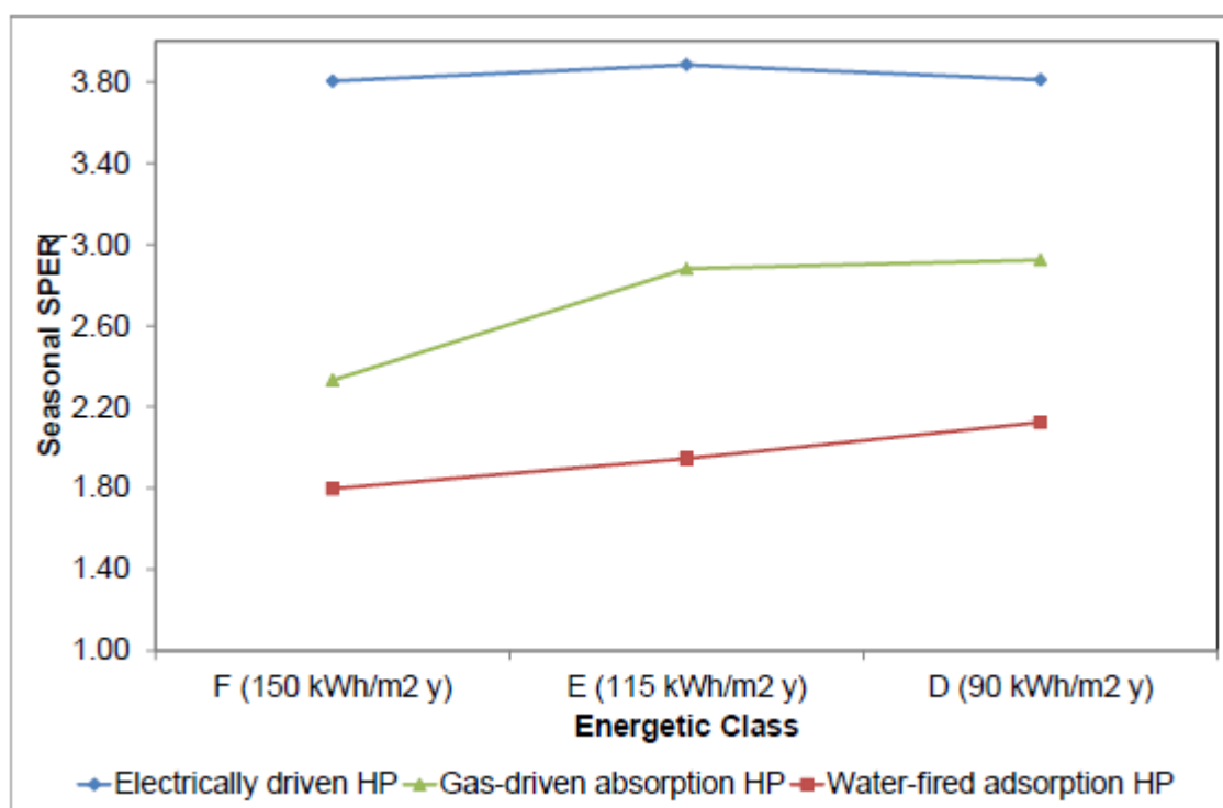
Figure 2: Comparison between the most performing simulated configurations for each heat pumping technology.
