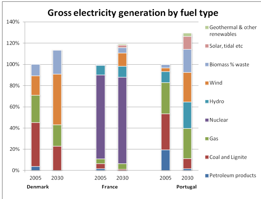
Figure 6-2 Electricity generation by fuel type for Denmark, France and Portugal. Figures of 2030 are depicted as percentages with regard to the demand in 2005. Source: DG-TREN forecast reports (Ref**).
