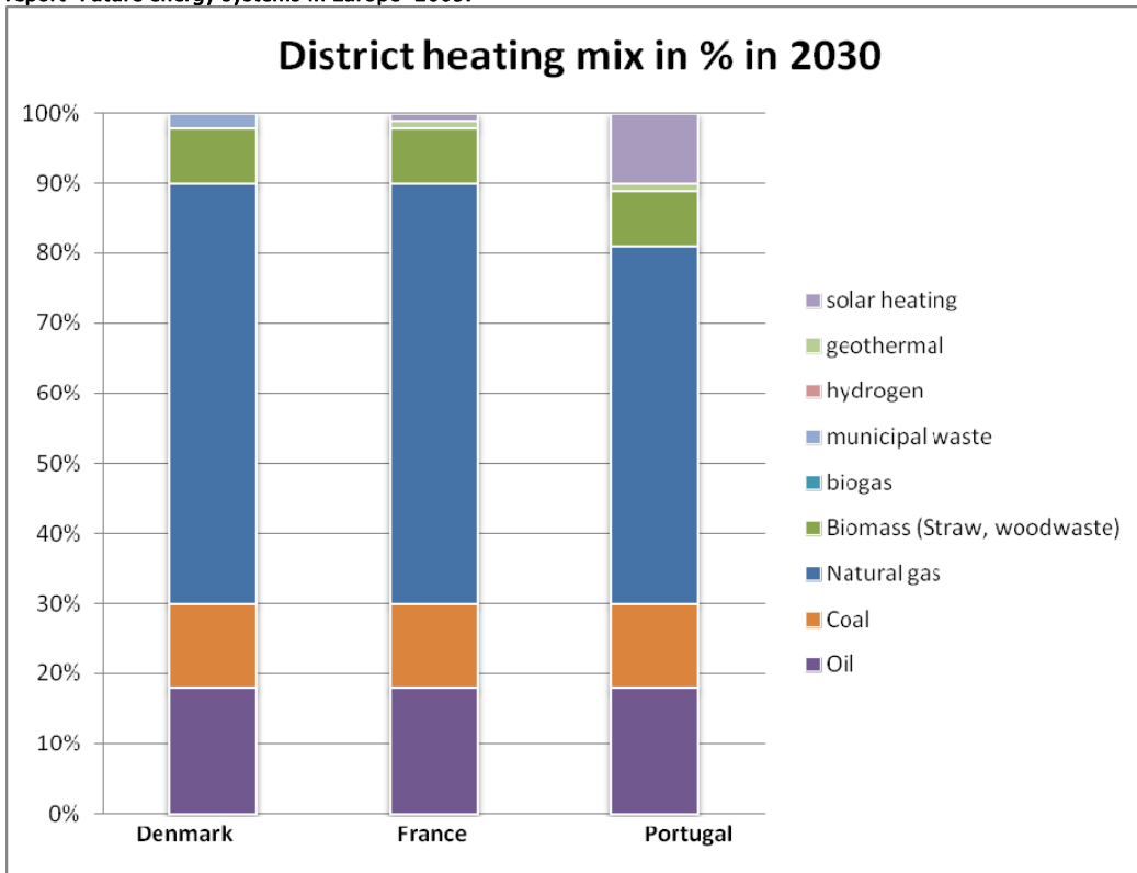
Figure 6-3 Fuel mix for district heating and CHP for Denmark, Portugal and France in 2030. Source: STOA report "Future energy systems in Europe" 2009.
